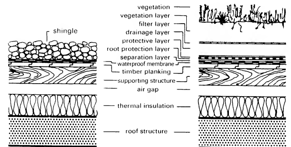
③ Cold roof → ④
